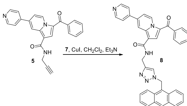
Scheme 1. Synthesis of compound 8 . Compounds 1 and 3 were reported earlier. 4a, 7a
