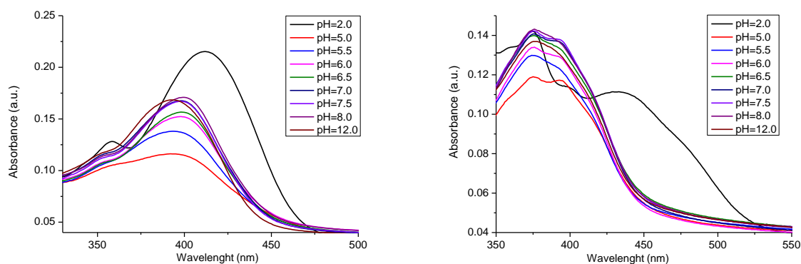
Fig. 2 UV-vis spectra in water for compound 5 (left) and 8 (right) at pH = 2.0 (0.1M, HCl); 5.0; 5.5; 6.0; 6.5; 7.0; 7.5; 8.0; 12.0 (0.1M, NaOH)
