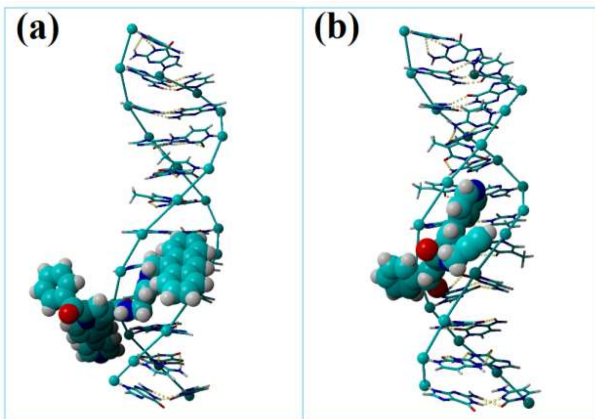
Fig. 6. Docking structures of the complexes between: (a) DNA oligonucleotide (receptor) and indolizine 8 (ligand): E_b = -9.87 kcal/mol and K_d = 58.138 nM; (b) DNA oligonucleotide (receptor) and indolizine 5 (ligand): E_b = -7.60 kcal/mol and K_d = 2681.6 nM.
