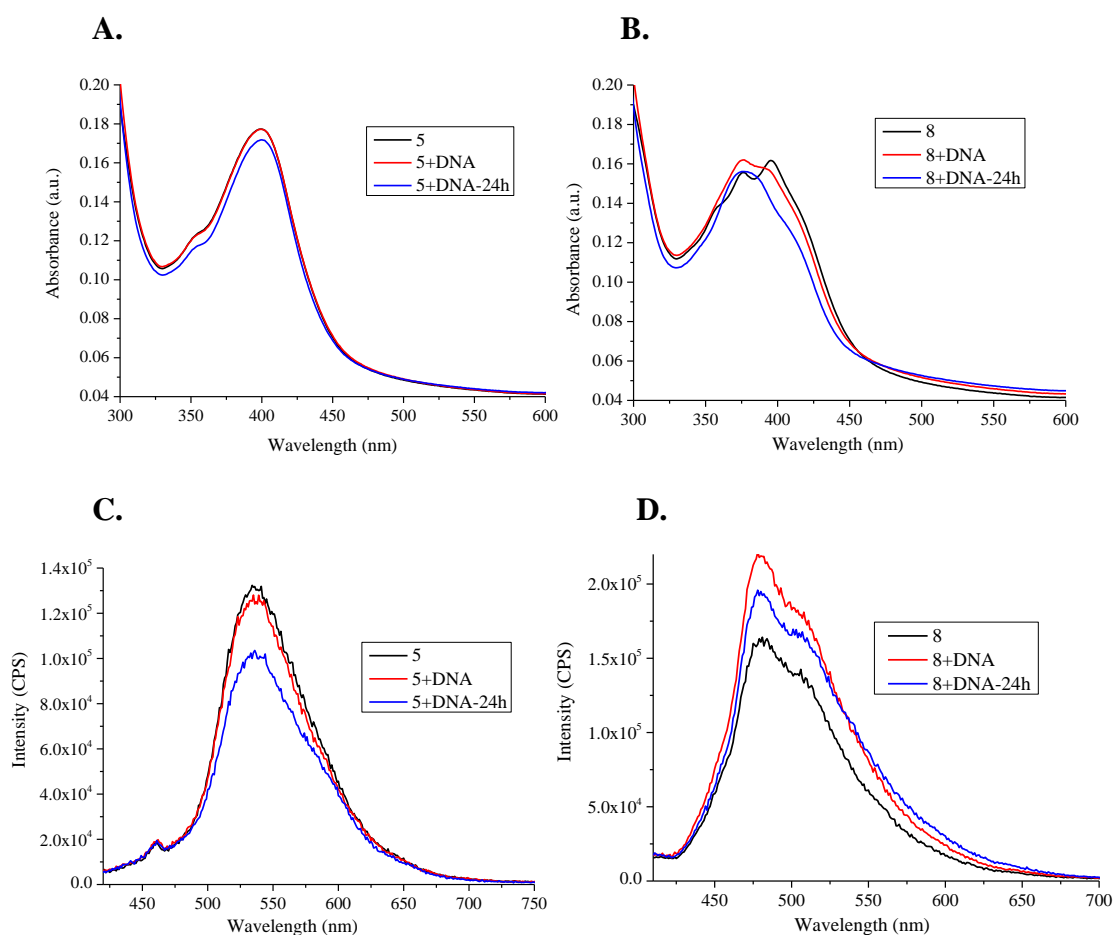
Fig. 5. UV-vis absorbance spectra of compounds 5 (A) and 8 (B) and fluorescence emission spectra of compounds 5 (C) and 8 (D) recorded at 22 °C in 1xTAE buffer pH 7.4 before and after the addition of DNA (0 min and 24 hours).
