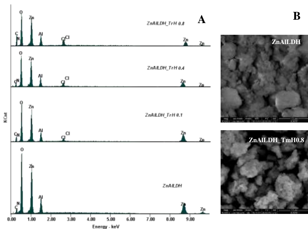
Fig. 3 - (A) EDX spectra of ZnAILDH, ZnAILDH_TrH 0.1, ZnAILDH_TrH 0.4 and ZnAILDH_TrH 0.8; (B) SEM micrograph for ZnAILDH and ZnAILDH_TrH 0.8
